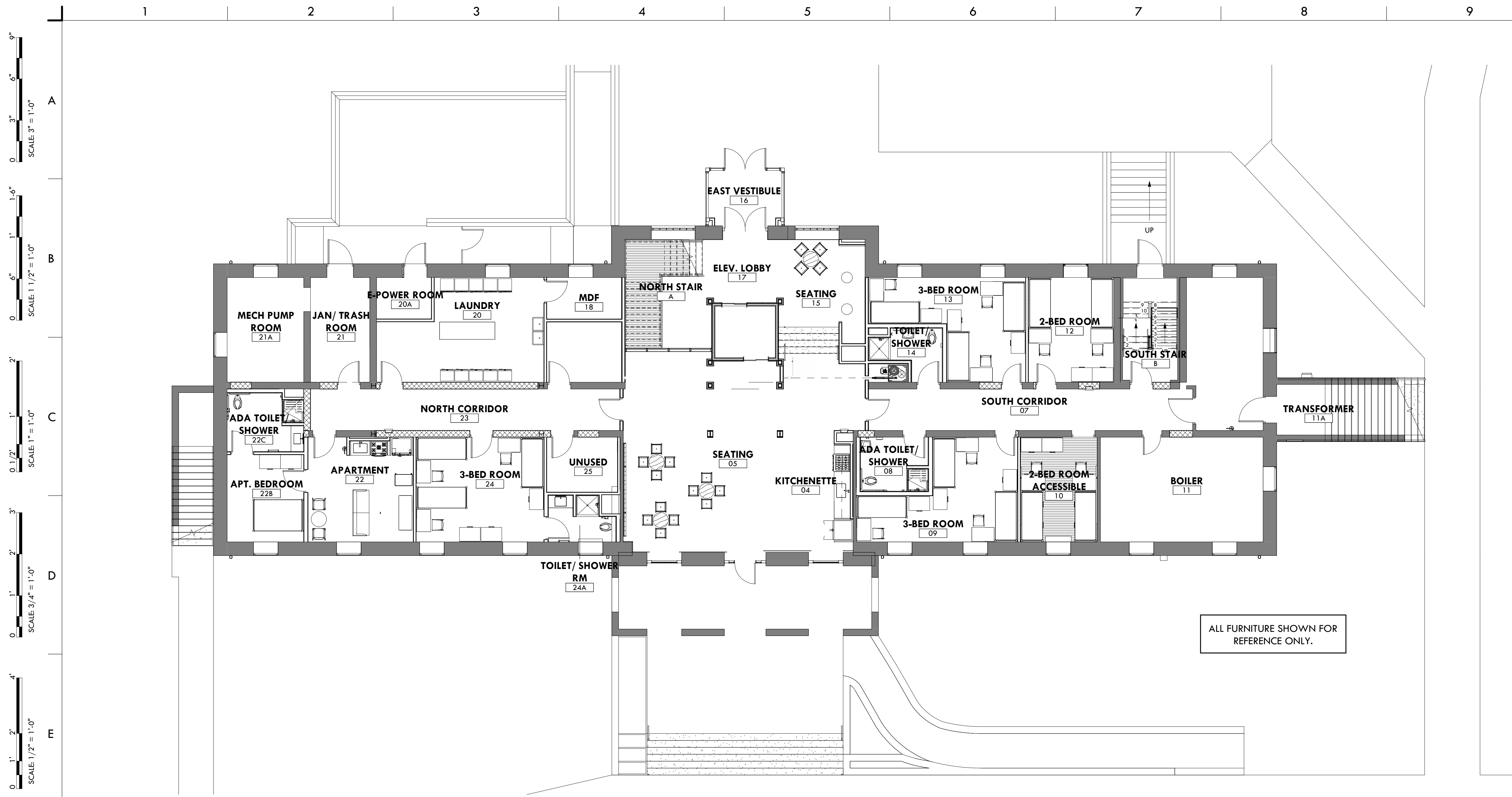
1 GROUND FLOOR FURNITURE PLAN
